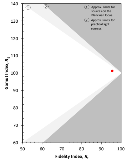
This plot shows a comparison of the R_t and R_g values relative to the range of possible values.
